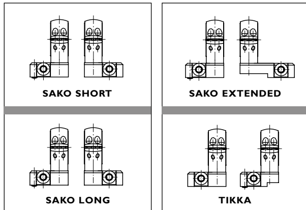
SAKO TRG QD OPTILOCK SCOPEMOUNT & SAKO OPTILOCK QUICKMOUNTS
